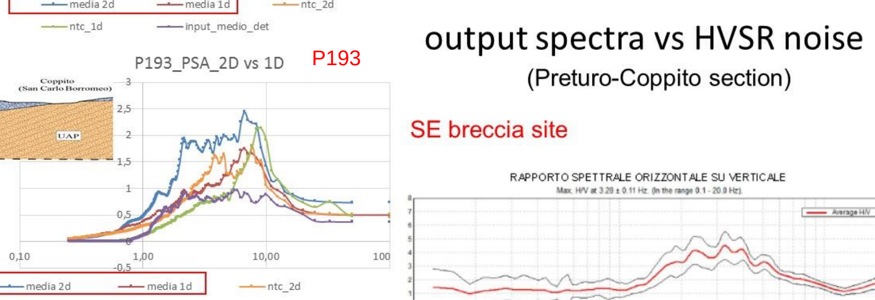
Fig. 8 - Output spectra (PSA vs frequency) vs HVSR noise. Left side: output spectra; blue and red curves refer to 2D (LSR) and 1D (EERA) modeling respectively. Right side: HVSR noise acquired nearby the local seismic response sites (P34, P127, P159, P193) (Preturo-Coppito section, Fig. 2).
