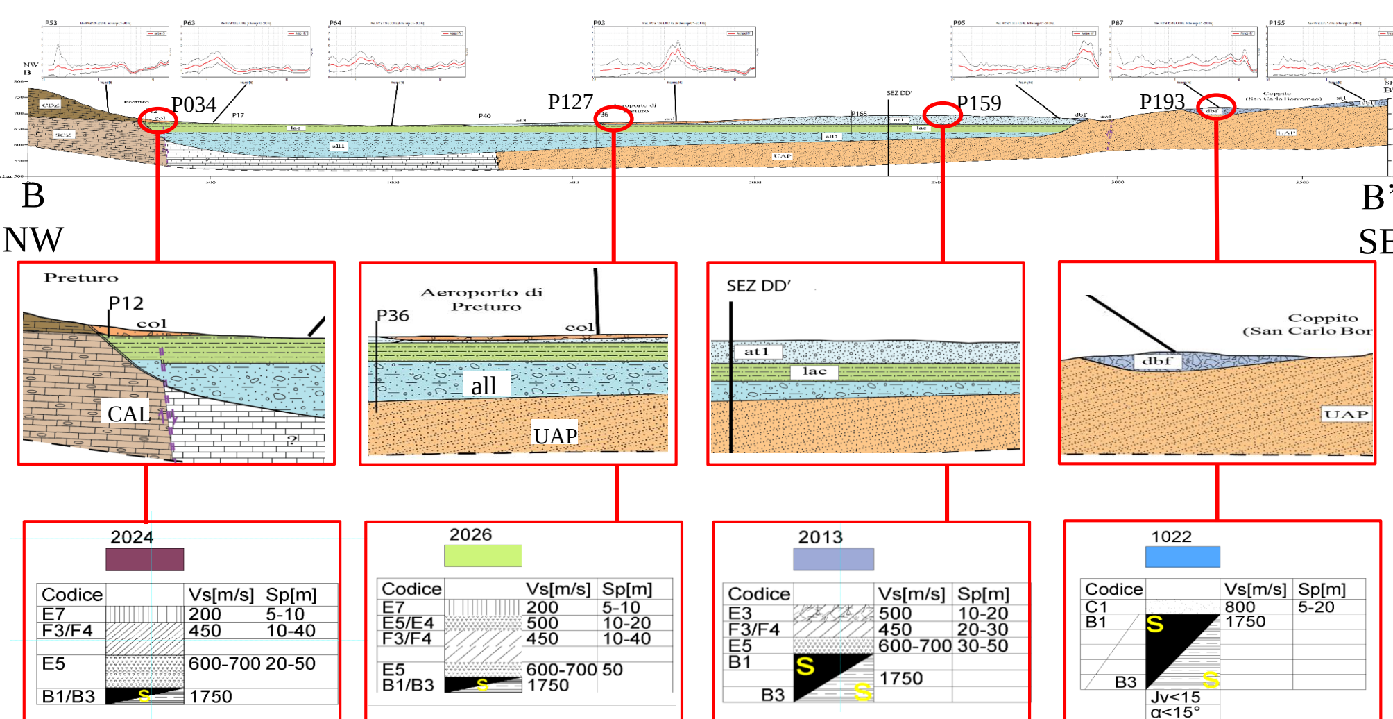
Fig. 2 - Preturo-Coppito geological section representative of the subsoil model of Western L'Aquila Plain (for the location see Fig. 2). Quaternary filling deposit: col: colluvium (Holocene); at1: terraced alluvium (Upper Pleistocene); dbf: calcareous breccia (Middle Pleistocene); lac: lacustrine clayey silt with lignite and sand (Lower Pleistocene); all: alluvium (gravel, sand, pelite) (Lower Pleistocene). Seismic bedrock: CAL: Miocene-Cretaceous limestone; UAP: Upper Miocene terrigenous unit (sandstone and claystone); Lithologies: B1/B3: layered rocks; C1: breccia; E3: sandy gravel; E4: sand; E5: gravelly sand; E7: sandy silt; F3: clayey silt; F4: silty clay; Sp: thickness; sites of 1D/2D simulations: P34 (NW valley edge); P127: valley center; P159 (SE valley edge); P193: breccia onto bedrock site.
