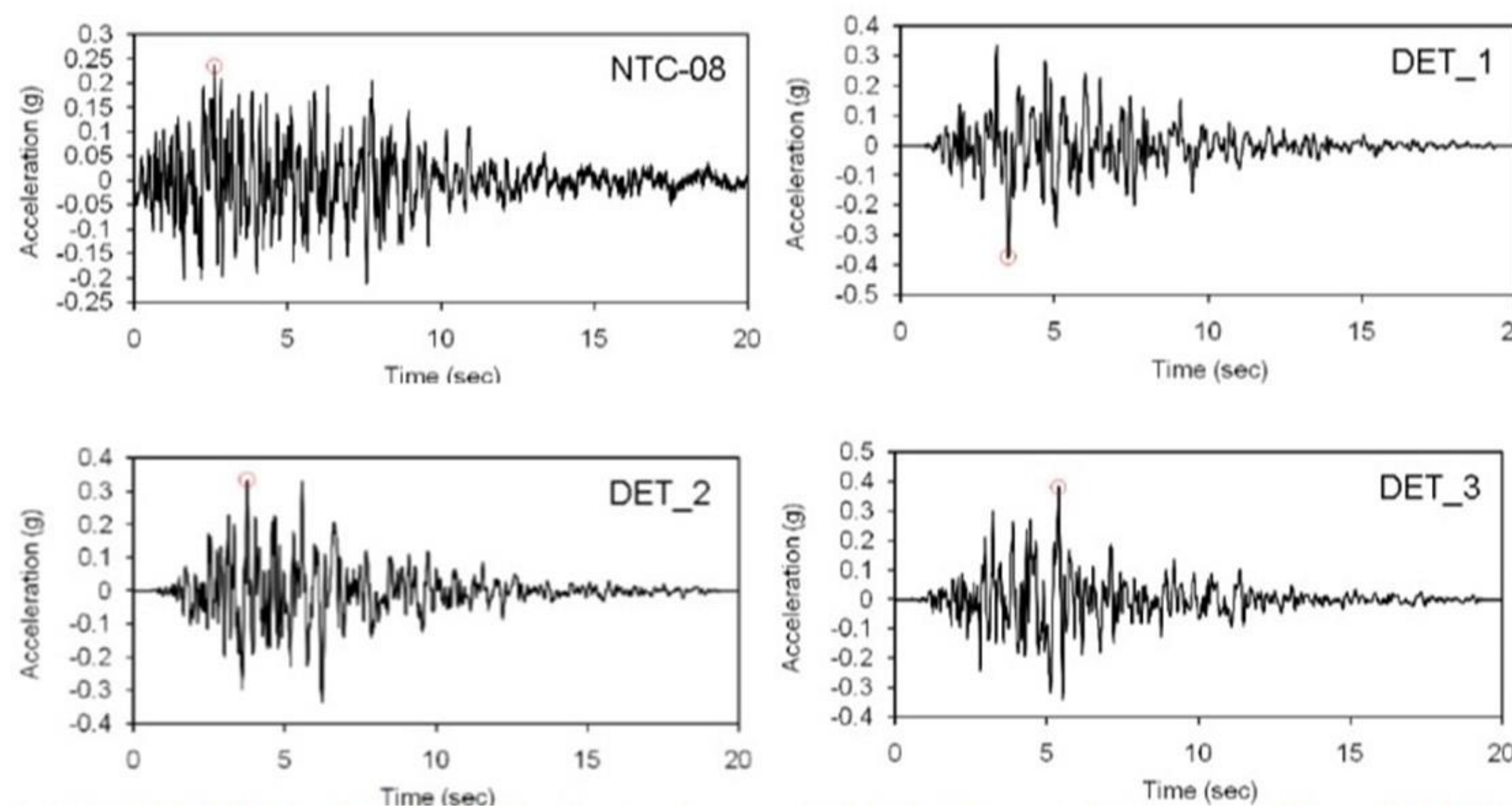
Fig. 3 – DET_1, DET_2, DET_3 and NTC-08 refer to the four accelerograms used in the 1D and 2D modeling (GdL MS-AQ, 2010).
