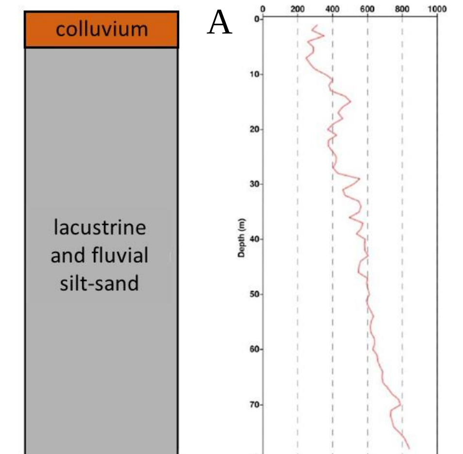
Fig. 6 - Geophysical in-hole tests to calibrate the Vs vs depth profile used in the modeling: cross-hole tests at Aterno R. bridge (Borgo Rivera, L'Aquila) (Cardarelli and Cercato, 2010) (A) and Colle dei Grilli - Cansatessa RAN section (Aterno R. Valley) (Lanzo et al., 2011) (B).
